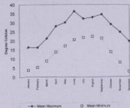
Average temp. in Muzaffarabad 1998.
